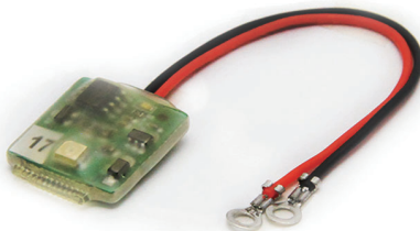
汎用ラグ端子<MiniZ MR03 RWD/Sports/Sports2 用>
