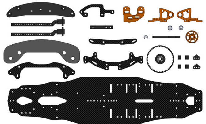
It is a main parts list. The upper bulk and the motor mount use 7075T6.
