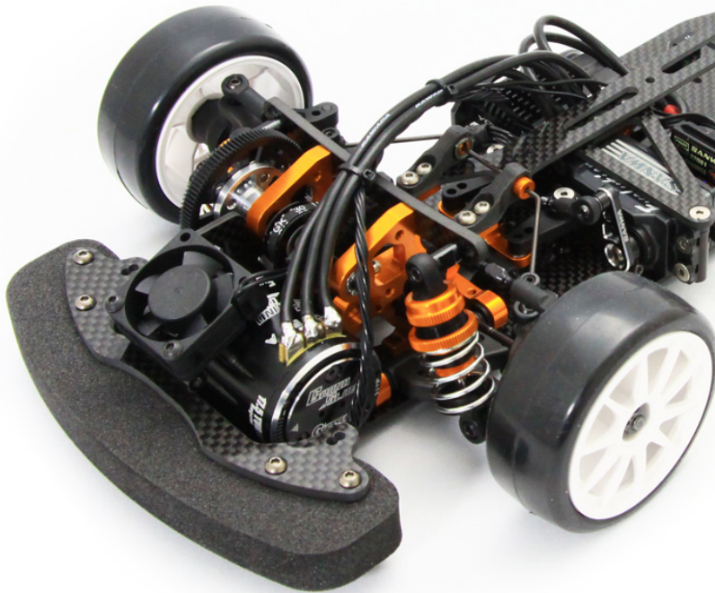
Battery Position1
